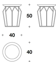
TCV (20) HIGH : SIDE TABLE Ø 40x50H.cm Ø 15 3/4x19 3/4H."
