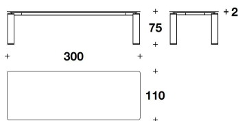
VTB (04) BIG : TAVOLO / TABLE 300x110x75H. - THK.2cm 118x43 1/3x29 2/3H. - THK.13/16"
