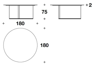
VTB (01) MEDIUM : TAVOLO TONDO / ROUND TABLE Ø 180x75H. - THK.2cm Ø 71x29 2/3H. - THK.13/16"
