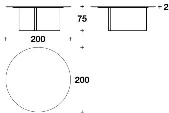
VTB (02) BIG : TAVOLO TONDO / ROUND TABLE Ø 200x75H. - THK.2cm Ø 78 2/3x29 2/3H. - THK.13/16"
