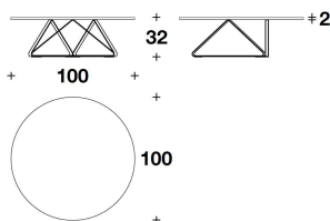
CTT (16) COFFEE TABLE Ø 100x32H.cm Ø 39 1/3x12 2/4H."
