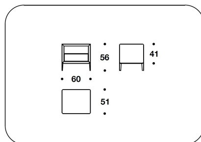
BCM (1R) CHESTNUT - BURR WALNUT : TAVOLO NOTTE / BEDSIDE TABLE 60x51x56H.cm 23 2/3x20x22H."
