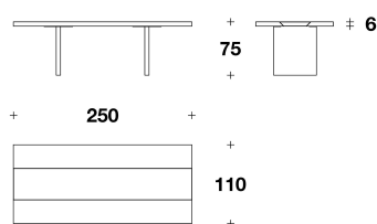
LLT (29E) TAVOLO RETTANGOLARE / RECTANGULAR TABLE 250x110x75H. - THK.6cm 98 1/3x43 1/3x29 2/3H. - THK.2 6/16"
