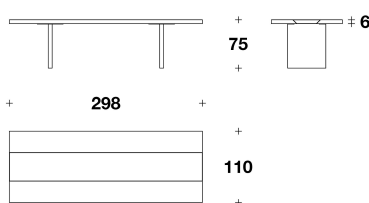
LLT (30E) TAVOLO RETTANGOLARE / RECTANGULAR TABLE 298x110x75H. - THK.6cm 117 1/3x43 1/3x29 2/3H. - THK.2 6/16"
