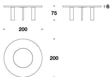
LLT (32E) TAVOLO TONDO / ROUND TABLE Ø 200x75H. - THK.6cm Ø 78 2/3x29 2/3H. - THK.2 6/16"
