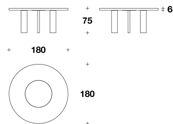
LLT (31E) TAVOLO TONDO / ROUND TABLE Ø 180x75H. - THK.6cm Ø 71x29 2/3H. - THK.2 6/16"
