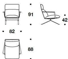
POT (5A) POLTRONA ALTA / HIGH ARMCHAIR 82x88x91H. - H.S.42cm 32 1/3x34 2/3x35 2/3H. - H.S.16 2/4"
