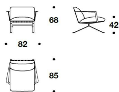
POT (5B) POLTRONA / ARMCHAIR 82x85x68H. - H.S.42 cm 32 1/3x33 1/3x26 2/3H. - H.S.16 2/4 "
