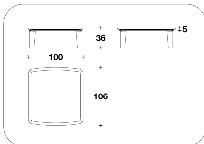
CTB (23PL) - CTB (23EL) - CTB (23EE) COFFEE TABLE 100x106x36H.cm 39 1/3x41 2/3x14 1/4H."
