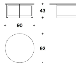
CTO (30V/1) - CTO (30V/1C) COFFEE TABLE 90x92x43H.cm 35 1/3x36 1/3x17H."
