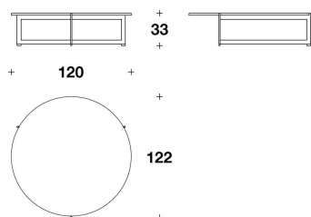
CTO (31V/1) - CTO (31V/1C) COFFEE TABLE 120x122x33H.cm 47 1/3x48x13H."
