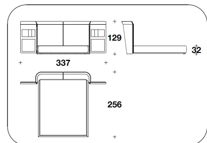
FET (CUSA) CALIFORNIA USA : LETTO PER MATERASSO / BED FOR MATTRESS 183x215 - 218x256x129H. - 337x256x129H. - H.B.32cm 72x84 2/3 - 85 2/3x100 2/3x50 2/3H. - 132 2/3x100 "
