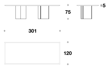
LLT (25M) MARBLE : TAVOLO RETTANGOLARE / RECTANGULAR TABLE 301x120x75H. - THK.5 cm 118 2/3x47 1/3x29 2/3H. - THK.1 15/16 "
