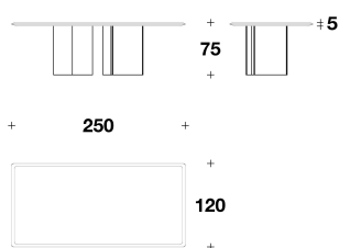
LLT (28M) MARBLE : TAVOLO RETTANGOLARE / RECTANGULAR TABLE 250x120x75H. - THK.5 cm 98 1/3x47 1/3x29 2/3H. - THK.1 15/16 "
