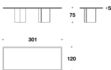
LLT (25E) - LLT (25V) TAVOLO RETTANGOLARE / RECTANGULAR TABLE 301x120x75H. - THK.5 cm 118 2/3x47 1/3x29 2/3H. - THK.1 15/16 "
