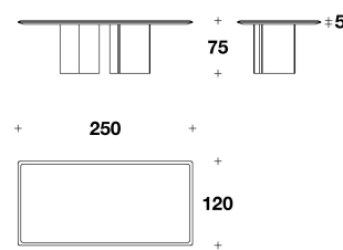
LLT (28E) - LLT (28V) TAVOLO RETTANGOLARE / RECTANGULAR TABLE 250x120x75H. - THK.5 cm 98 1/3x47 1/3x29 2/3H. - THK.1 15/16 "
