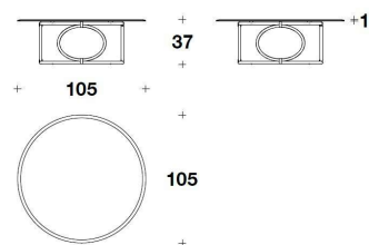
CTT (22V) - CTT (22M) COFFEE TABLE Ø 105x37H.cm Ø 41 1/3x14 2/4H."
