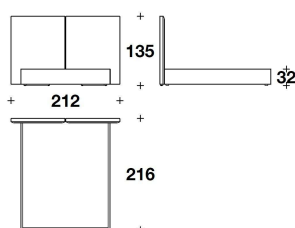
LFD (LE1) LETTO PER MATERASSO / BED FOR MATTRESS 165x200 - 212x216x135H. - H.B.32cm 65x78 2/3 - 83 1/3x85x53H. - H.B.12 2/4"
