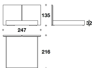
LFD (LE7) LETTO PER MATERASSO / BED FOR MATTRESS 200x200 - 247x216x135H. - H.B.32cm 78 2/3x78 2/3 - 97 1/3x85x53H. - H.B.12 2/4"
