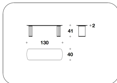
CTB (29ME) - CTB (29MP) MARBLE : COFFEE TABLE 130x40x41H.cm 51 1/3x15 3/4x16 1/4H."
