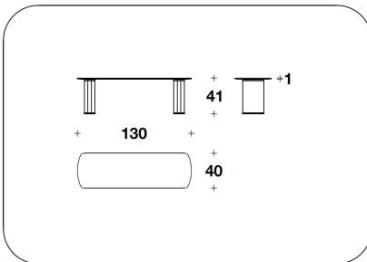
CTB (29PE) - CTB (29PP) - CTB (29VE) - CTB (29VP) COFFEE TABLE 130x40x41H.cm 51 1/3x15 3/4x16 1/4H."
