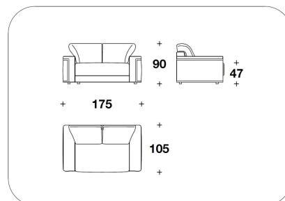
MNG (LS) LOVESEAT 175x105x90H. - H.S.47cm 69x41 1/3x35 1/3H. - H.S.18 2/4"
