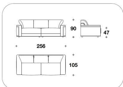
MNG (D3) DIVANO 3 POSTI / 3 SEATER SOFA 256x105x90H. - H.S.47cm 100 2/3x41 1/3x35 1/3H. - H.S.18 2/4"
