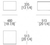
Hanging night table W. 480 mm
