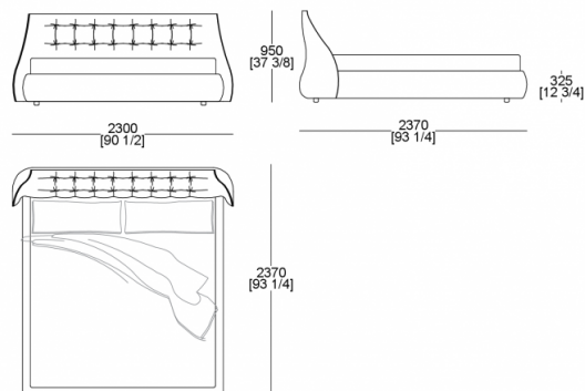
Bed (mattress W. 1930 x D. 2020 mm)
