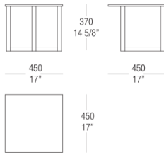
Small table W. 450 lacquered top
