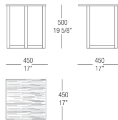
Small table W. 450 wood top
