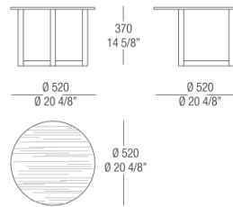
Small table Ø 520 wood top
