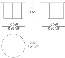
Small table Ø 520 leather top
