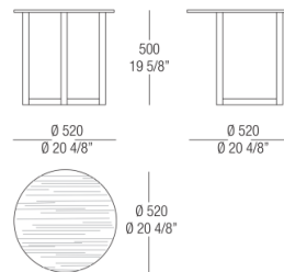
Small table Ø 520 wood top
