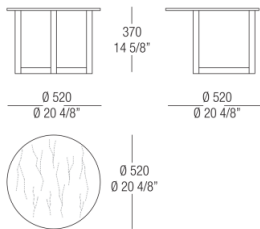
Small table Ø 520 marble top
