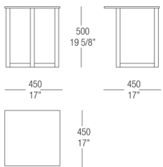
Small table W. 450 lacquered top
