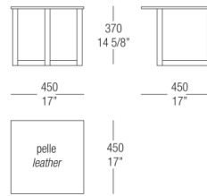
Small table W. 450 leather top
