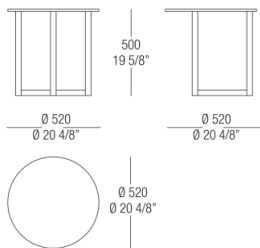
Small table Ø 520 lacquered top
