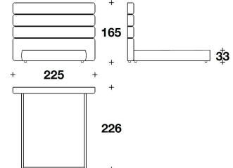
NBR (LE1) HIGH : LETTO PER MATERASSO / BED FOR MATTRESS 165x200 - 225x226x165H. - H.B.33 cm 65x78 2/3 - 88 2/3x89x65H. - H.B.13 "
