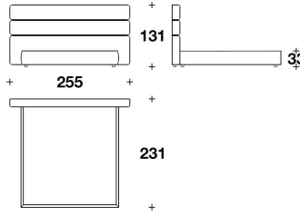
NBR (BKUSA) KING USA : LETTO PER MATERASSO / BED FOR MATTRESS 195x205 - 255x231x131H. - H.B.33 cm 76 2/3x80 2/3 - 100 1/3x91x51 2/3H. - H.B.13 "
