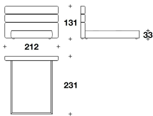
NBR (BQUSA) QUEEN USA : LETTO PER MATERASSO / BED FOR MATTRESS 152x205 - 212x231x131H. - H.B.33 cm 60x80 2/3 - 83 1/3x91x51 2/3H. - H.B.13 "
