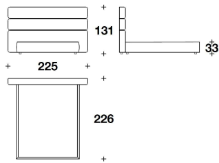
NBR (BLE1) LETTO PER MATERASSO / BED FOR MATTRESS 165x200 - 225x226x131H. - H.B.33 cm 65x78 2/3 - 88 2/3x89x51 2/3H. - H.B.13 "
