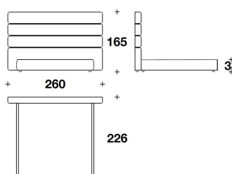
NBR (LE7) HIGH : LETTO PER MATERASSO / BED FOR MATTRESS 200x200 - 260x226x165H. - H.B.33 cm 78 2/3x78 2/3 - 102 1/3x89x65H. - H.B.13 "
