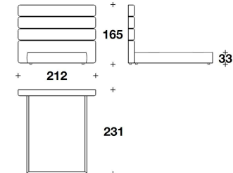
NBR (QUSA) HIGH - QUEEN USA : LETTO PER MATERASSO / BED FOR MATTRESS 152x205 - 212x231x165H. - H.B.33 cm 60x80 2/3 - 83 1/3x91x65H. - H.B.13 "
