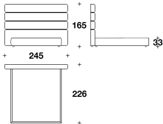
NBR (LE2) HIGH : LETTO PER MATERASSO / BED FOR MATTRESS 185x200 - 245x226x165H. - H.B.33 cm 73x78 2/3 - 96 1/3x89x65H. - H.B.13 "
