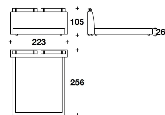
ELN (CUSA) CALIFORNIA USA : LETTO PER MATERASSO / BED FOR MATTRESS 183x215 - 223x256x105H. - H.B.26cm 72x84 2/3 - 87 2/3x100 2/3x41 1/3H. - H.B.10 1/4"
