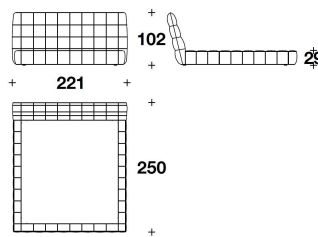
NIO (LE2) LETTO PER MATERASSO / BED FOR MATTRESS 185x200 - 221x250x102H. - H.B.29cm 73x78 2/3 - 87x98 1/3x40H. - H.B.11 2/4"
