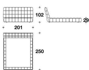
NIO (LE1) LETTO PER MATERASSO / BED FOR MATTRESS 165x200 - 201x250x102H. - H.B.29cm 65x78 2/3 - 79x98 1/3x40H. - H.B.11 2/4"
