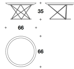
TCV (10) BIG : COFFEE TABLE Ø 66x35H.cm Ø 26x13 3/4H."
