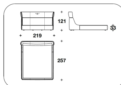
LB1 (CUSA) CALIFORNIA USA : LETTO PER MATERASSO / BED FOR MATTRESS 183x215 - 219x257x121H. - H.B.33cm 72x84 2/3 - 86 1/3x101 1/3x47 2/3H. - H.B.13"
