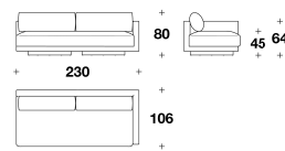
RHS (ED) - RHS (ES) ELEMENTO SEDUTA CON BRACCIOLO DX O SX / SEAT ELEMENT WITH RIGHT OR LEFT ARMREST 230x106x80H. - H.A.64 - H.S.45 cm 90 2/3x41 2/3x31 1/3H. - H.A.25 1/3 - H.S.17 3/4 "
