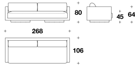
RHS (D4) DIVANO 4 POSTI / 4 SEATER SOFA 268x106x80H. - H.A.64 - H.S.45 cm 105 2/3x41 2/3x31 1/3H. - H.A.25 1/3 - H.S.17 3/4 "
