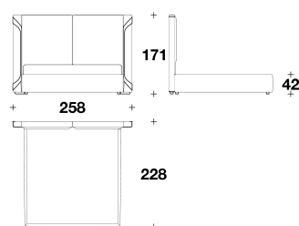
ICN (KUSA) KING USA : LETTO PER MATERASSO / BED FOR MATTRESS 195x205 - 258x228x171H. - H.B.42 cm 76 2/3x80 2/3 - 101 2/3x89 2/3x67 1/3H. - H.B.16 2"
