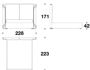
ICN (LE1) LETTO PER MATERASSO / BED FOR MATTRESS 165x200 - 228x223x171H. - H.B.42 cm 65x78 2/3 - 89 2/3x87 2/3x67 1/3H. - H.B.16 2/4 "
