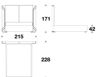
ICN (QUSA) QUEEN USA : LETTO PER MATERASSO / BED FOR MATTRESS 152x205 - 215x228x171H. - H.B.42 cm 60x80 2/3 - 84 2/3x89 2/3x67 1/3H. - H.B.16 2/4 "
