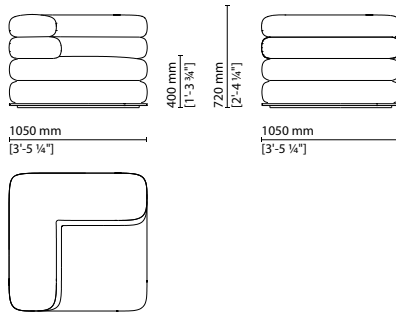
078 018 — Right corner element
