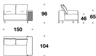
1CO (E1GD) - 1CO (E1GS) BIG : ELEMENTO 1 POSTO CON BRACCIOLO DX O SX / 1 SEATER ELEMENT WITH RIGHT OR LEFT ARMREST 150x104x96H. – H.S.46cm 59x41x37 2/3H. – H.S.18"
