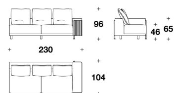
1CO (E2MD) - 1CO (E2MS) MEDIUM : ELEMENTO 2 POSTI CON BRACCIOLO DX O SX / 2 SEATER ELEMENT WITH RIGHT OR LEFT ARMREST 230x104x96H. – H.S.46cm 90 2/3x41x37 2/3H. – H.S.18"
