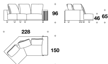
1CO (ANGD) - 1CO (ANGS) ELEMENTO ANGOLARE INCLINATO CON BRACCIOLO DX O SX / CURVED CORNER ELEMENT WITH RIGHT OR LEFT ARMREST 228x150x96H. – H.S.46cm 89 2/3x59x37 2/3H. – H.S.18"
