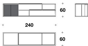
LLM (17B) MOBILE TV / TV CABINET 240x60x60H. cm 94 1/3x23 2/3x23 2/3H. "
