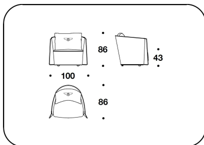
BTF (POL) POLTRONA / ARMCHAIR 100x86x86H. - H.S.43cm 39 1/3x34x34H. - H.S.17"
