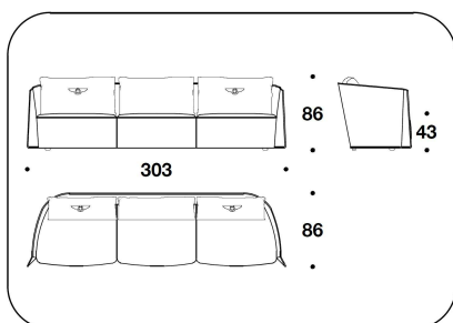
BTF (D4) DIVANO 4 POSTI / 4 SEATER SOFA 303x86x86H. - H.S.43cm 119 1/3x34x34H. - H.S.17"
