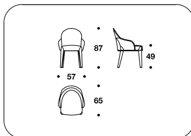
SEF (26B) SEDIA CON BRACCIOLI / CHAIR WITH ARMRESTS 57x65x87H. - H.S.49cm 22 1/3x25 2/3x34 1/3H. - H.S.19 1/4"
