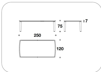
BTV (15VL) - BTV (15EL) - BTV (15EE) TAVOLO / TABLE 250x120x75H. - THK.7cm 98 1/3x47 1/3x29 2/3H. - THK.2 3/4"
