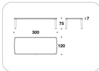
BTV (16VL) - BTV (16EL) - BTV (16EE) TAVOLO / TABLE 300x120x75H. - THK.7cm 118x47 1/3x29 2/3H. - THK.2 3/4"
