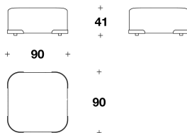
PF1 (02M) SQUARE : POUF / OTTOMAN 90x90x41H. cm 35 1/3x35 1/3x16 1/4H. "
