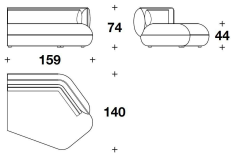
WAI (PEDB) - WAI (PESB) ELEMENTO PENISOLA 1 POSTO CON BRACCIOLO DX O SX / 1 SEATER PENISULA ELEMENT WITH RIGHT OR LEFT ARMREST 159x140x74H. - H.S.44cm 62 2/3x55x29H. - H.S.17 1/4"
