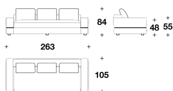
BRT (D3) DIVANO 3 POSTI / 3 SEATER SOFA 263x105x84H. - H.A.55 - H.S.48 cm 103 2/3x41 1/3x33H. - H.A.21 2/3 - H.S.19 "
