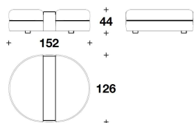
BRT (POUT1) ISOLA / ISLAND 152x126x44H.cm 60x49 2/3x17 1/4H."
