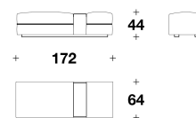
BRT (POUR) POUF RETTANGOLARE / RECTANGULAR OTTOMAN 172x64x44H. cm 67 2/3x25 1/3x17 1/4H. "
