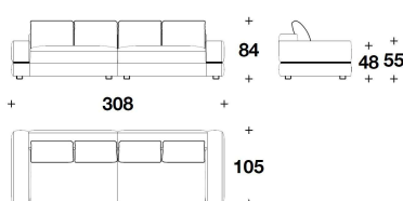
BRT (D4) DIVANO 4 POSTI IN 2 ELEMENTI / 4 SEATER SOFA IN 2 ELEMENTS 308x105x84H. - H.A.55 - H.S.48 cm 121 1/3x41 1/3x33H. - H.A.21 2/3 - H.S.19 "
