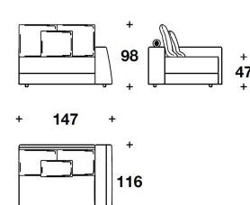
ELN (AE1D) - ELN (AE1S) ELEMENTO 1 POSTO CON BRACCIOLO DX O SX / 1 SEATER ELEMENT WITH RIGHT OR LEFT ARMREST 147x116x98H. - H.S.47cm 58x45 2/3x38 2/3H. - H.S.18 2/4"
