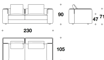
GON (A3BRD) - GON (A3BRS) DIVANO ANGOLARE 3 POSTI CON BRACCIOLO DX O SX / 3 SEATER CORNER SOFA WITH RIGHT OR LEFT ARMREST 230x105x90H. – H.S.47cm 90 2/3x41 1/3x35 1/3H. – H.S.18 2/4"
