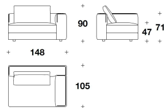
GON (EDG) - GON (ESG) BIG : ELEMENTO 1 POSTO CON BRACCIOLO DX O SX / 1 SEATER ELEMENT WITH RIGHT OR LEFT ARMREST 148x105x90H. – H.S.47cm 58 1/3x41 1/3x35 1/3H. – H.S.18 2/4"
