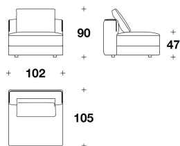
GON (E1C) ELEMENTO CENTRALE 1 POSTO / 1 SEATER CENTRAL ELEMENT 102x105x90H. – H.S.47cm 40x41 1/3x35 1/3H. – H.S.18 2/4"
