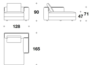
GON (CLD) - GON (CLS) CHAISE LONGUE 1 POSTO CON BRACCIOLO DX O SX / 1 SEATER CHAISE LONGUE WITH RIGHT OR LEFT ARMREST 128x165x90H. – H.S.47cm 50 1/3x65x35 1/3H. – H.S.18 2/4"
