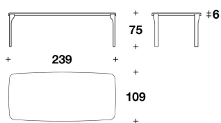
TTV (21MP) - TTV (21PP) LEATHER : TAVOLO / TABLE 239x109x75H. - THK.6cm 94x43x29 2/3H. - THK.2 6/16"
